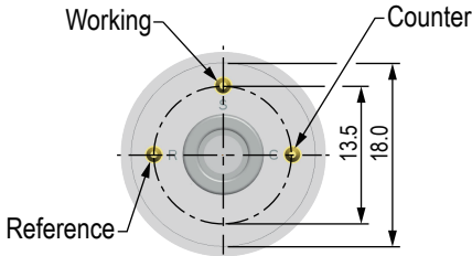
All dimensions in mm All tolerances \pm 0.20 mm unless otherwise stated
